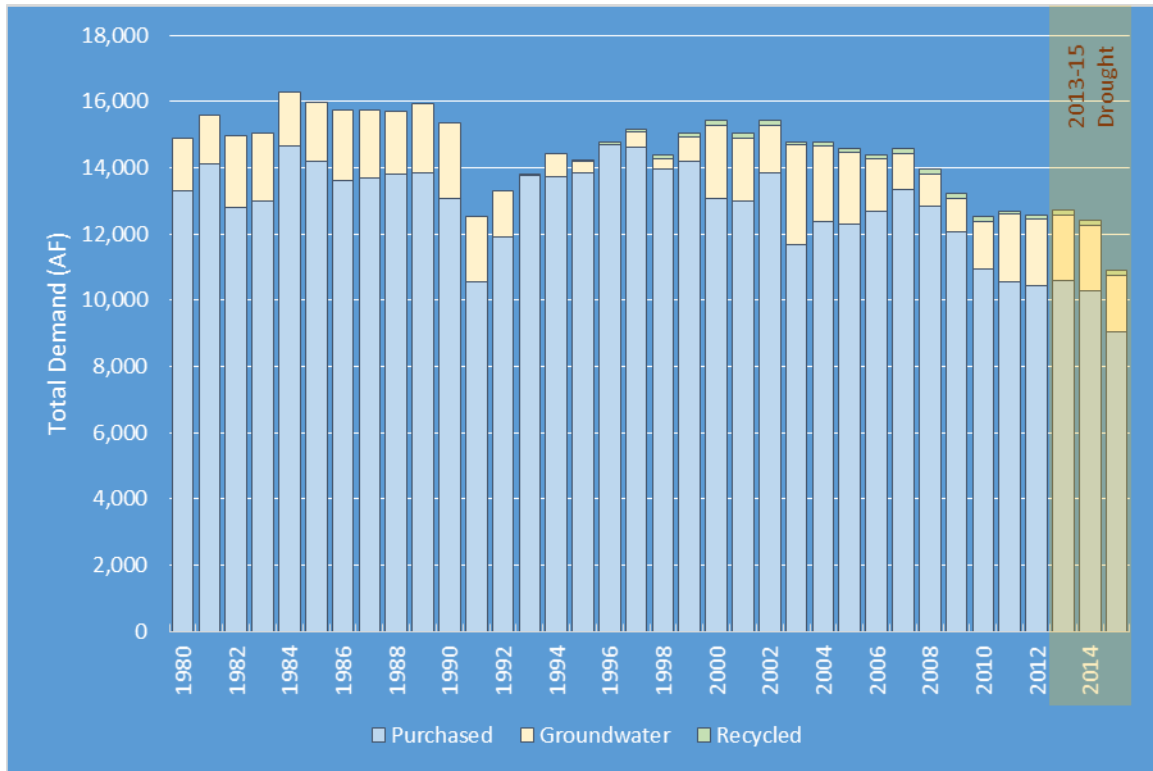
Figure 4. Hermosa-Redondo District Total Demand and Sources of Supply: 1980 - 2015
