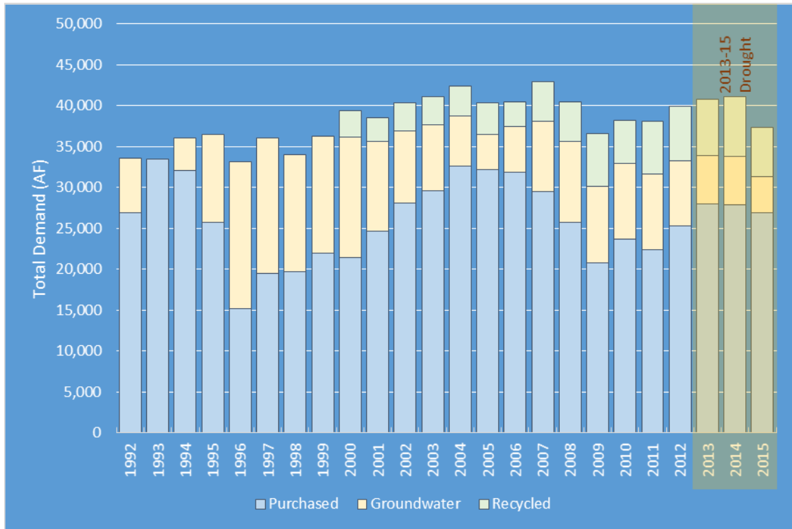
Figure 4. Dominguez District Total Demand and Sources of Supply: 1992 - 2015
