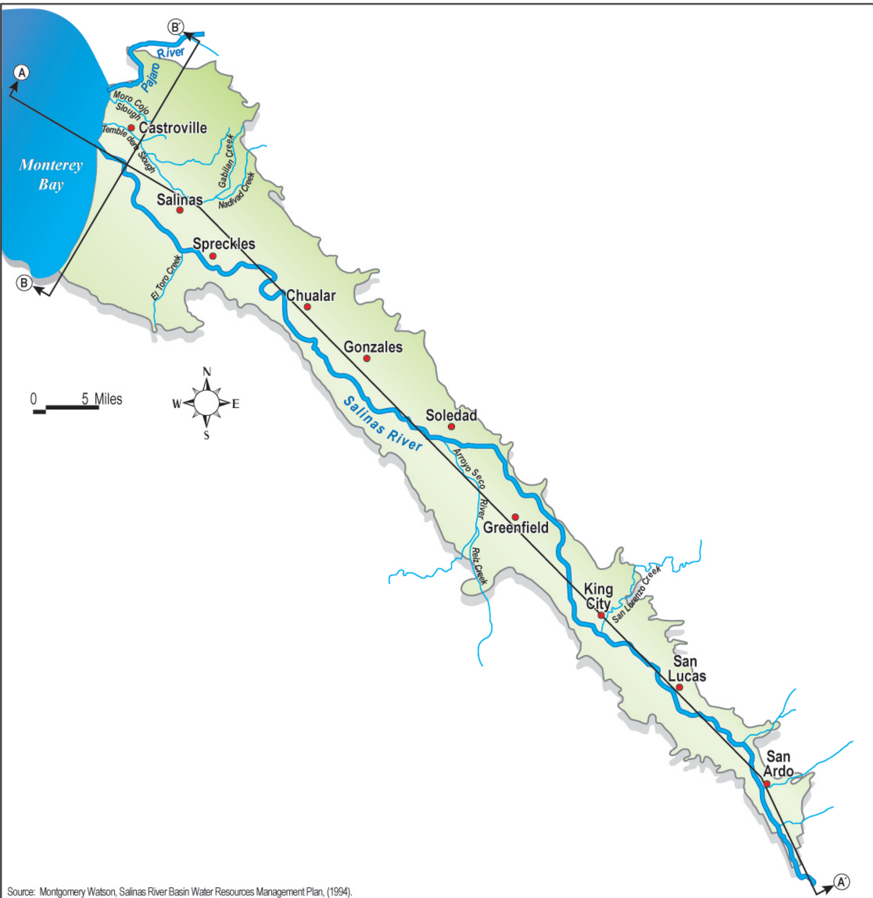
Figure 3-2: Location of Schematic Geologic Cross-Sections
