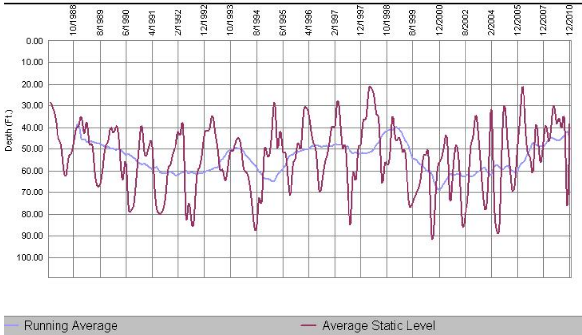
Figure 4.4-1: District Well Level Average (Static) District: DIXON For All Years As Of: 1/21/2011
