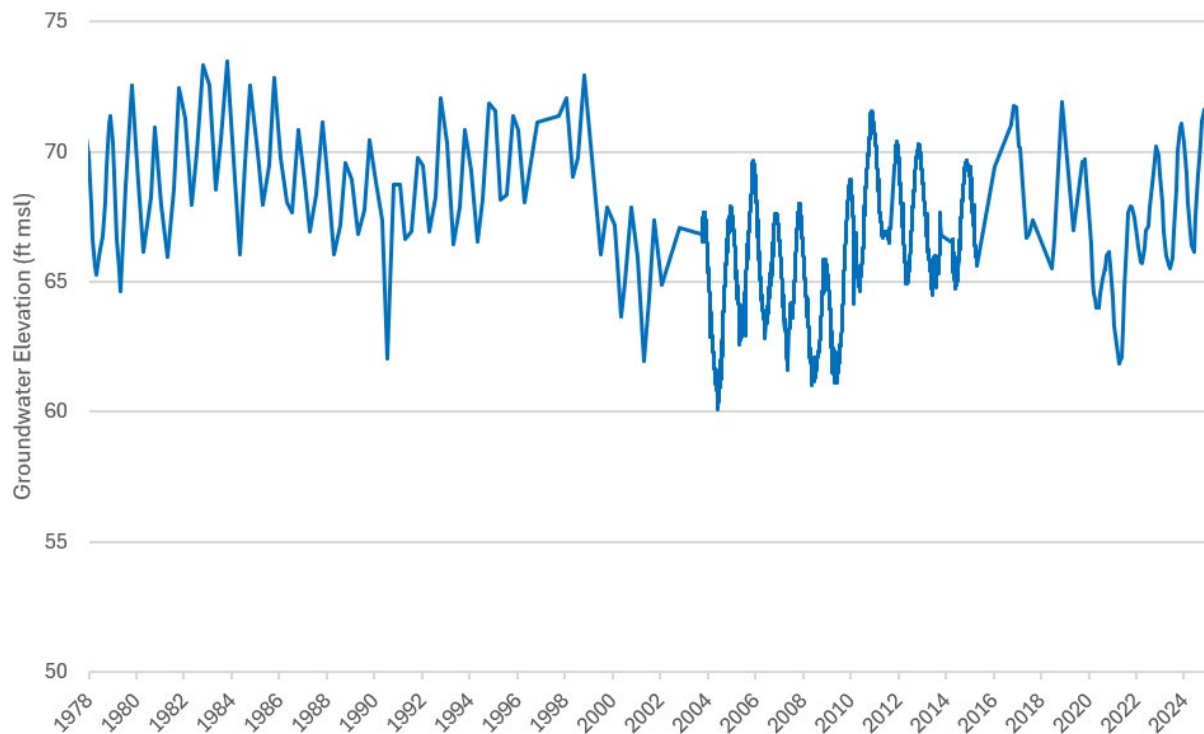
Figure 7-1. Groundwater Level Trend at Monitoring Well SRP0357 42
