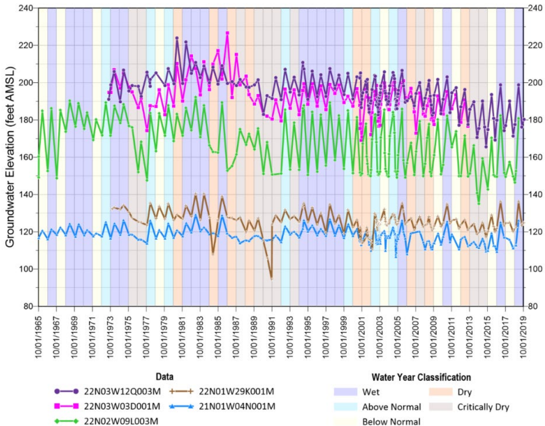
Figure 7-1. South Area Characteristic Hydrographs (GSP Figure 3-27)
