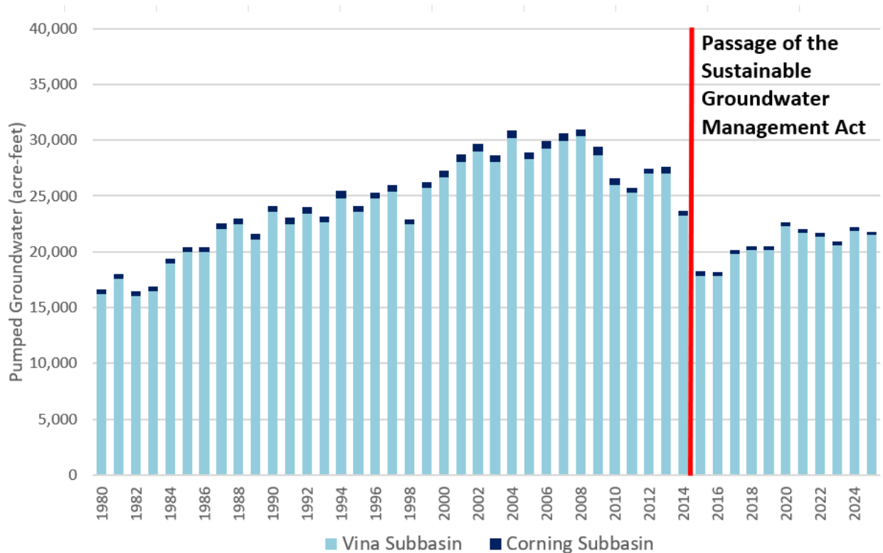
Figure 6-2. Historical Pumping from Groundwater Basins Underlying the Chico-Hamilton City District
