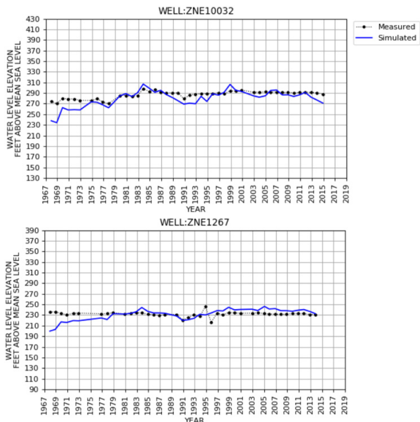
Figure 7-1. Hydrographs for Wells North of King City
