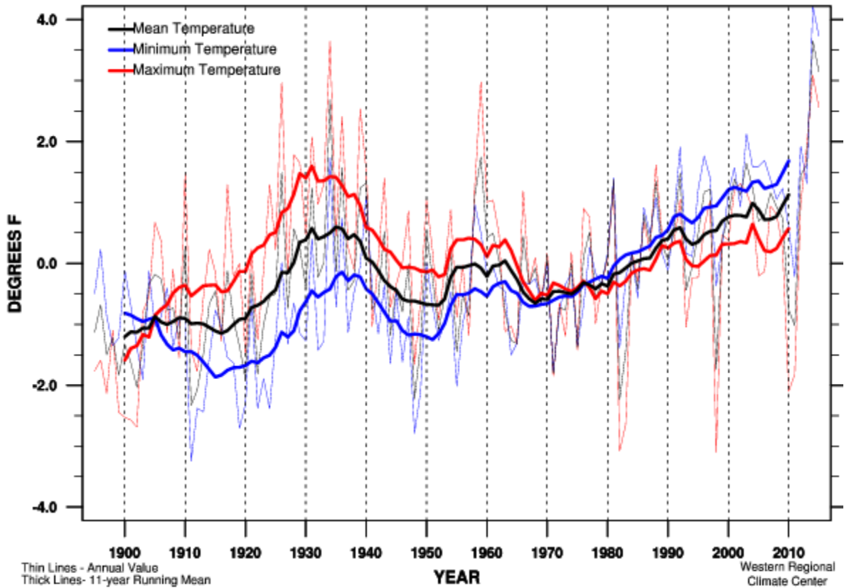
Figure 3-6. Temperature Departure, Sierra Region
